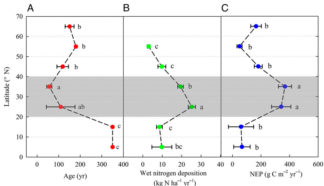
Fig. 5. Latitudinal distribution of NEP, wet nitrogen deposition and forest age in the Asian region. ( A ) The latitudinal distribution of forest age for Asian forest ecosystems between 0°N and 70°N. n = 2, 2, 4, 12, 9, 2, 4 , respectively, for seven bins from 0°N to 70°N. ( B ) The latitudinal distribution of wet nitrogen deposition for Asian forest ecosystems between 0°N and 70°N. n = 4, 13, 98, 80, 20, 5 , respectively, for six bins from 0°N to 60°N. ( C ) The latitudinal distribution of NEP for the Asian forest ecosystems between 0°N and 70°N. n = 2, 2, 4, 14, 9, 2, 4 , respectively, for the seven bins from 0°N to 70°N. The circles and bars represent the mean \pm 1 SE for 10° latitude bins. The values that differ significantly are labeled with different lowercase letters, marked as a, b, and c, successively ( P < 0.05 ).
